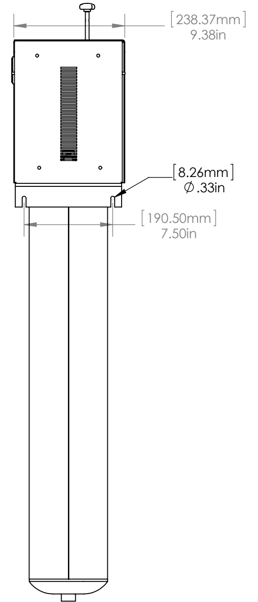
BACK VIEW
